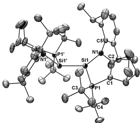
Figure 1. Molecular structure of 2 . Thermal ellipsoids represent 30% probability. H atoms are omitted for clarity. Selected bond lengths [Å], angles, and torsion angles [°]: Si1–Si1' 2.3306(12), Si1–P1 2.3274(9), P1–C1 1.760(2), C1–C2 1.375(3), C2–N1 1.360(3), Si1–N1 1.8805(18); P1–Si1–Si1' 103.64(4), N1–Si1–Si1' 137.60(6), N1–Si1–P1 88.41(6), Si1–P1–C1 93.03(8), P1–C1–C2 115.52(17), C1–C2–N1 124.97(19), C2–N1–Si1 113.65(14), C2–N1–C5 118.57(17), C5–N1–Si1 117.03(14), N1–Si1–Si1'–N1 4.86, P1–Si1–Si1'–P1' 159.10.
